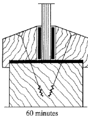
Typical sections through proprietary glazing systems using intumescent seals
